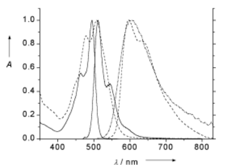
Figure 1. UV/Vis absorption and fluorescence spectra of 3b in dichloromethane (—) and as thin film (---) on a quartz substrate and film emission spectrum of 3c (•••).
